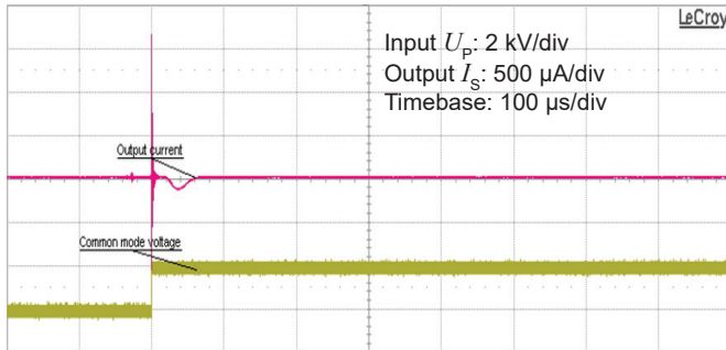
Figure 13: Typical common mode perturbation (2000 V step with 6 \text{ kV}/\mu\text{s} , R_M = 100 \Omega )
