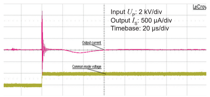
Figure 14: Detail of typical common mode perturbation (2000 V step with 6 \text{ kV}/\mu\text{s} , R_M = 100 \Omega )
