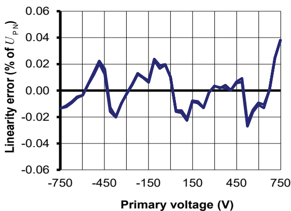
Figure 16: Typical linearity error at 25^\circ\text{C}
